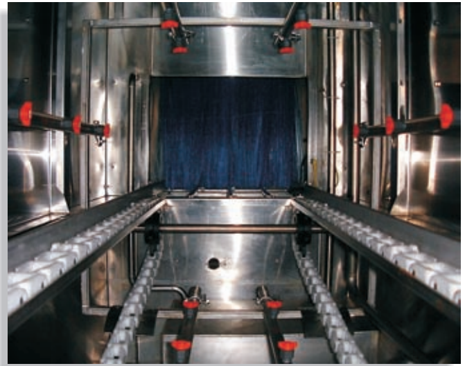
A typical wash section, showing quick pick-off jets
